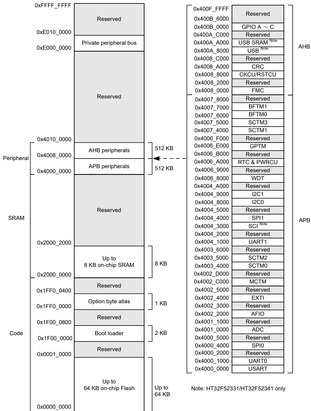
Figure 2. Memory Map
