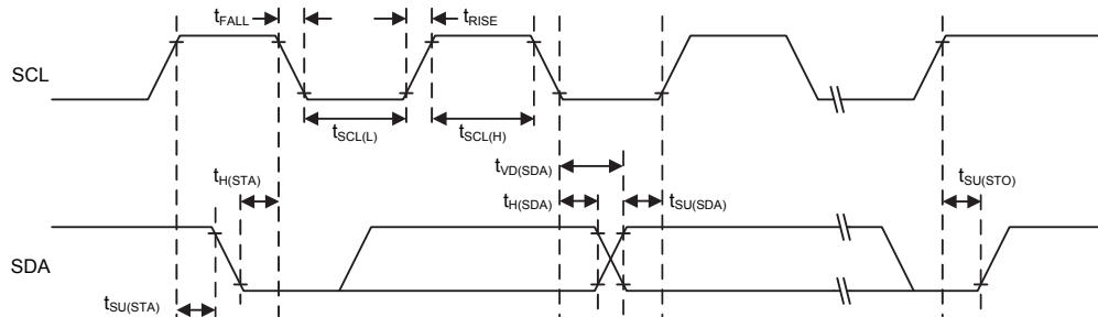
Figure 11. I²C Timing Diagrams
