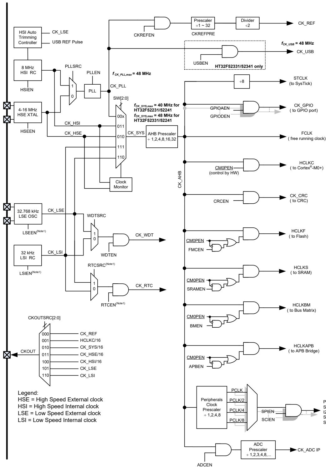
Figure 3. Clock Structure
