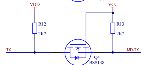
Level Shift Circuit
