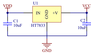
LDO Circuit
